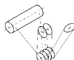
Modeltype 4/2 – Z
